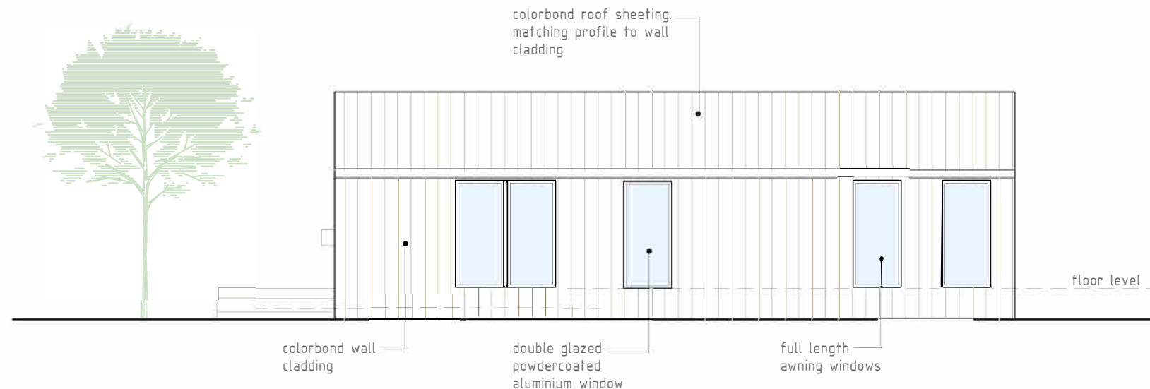
rear elevation
